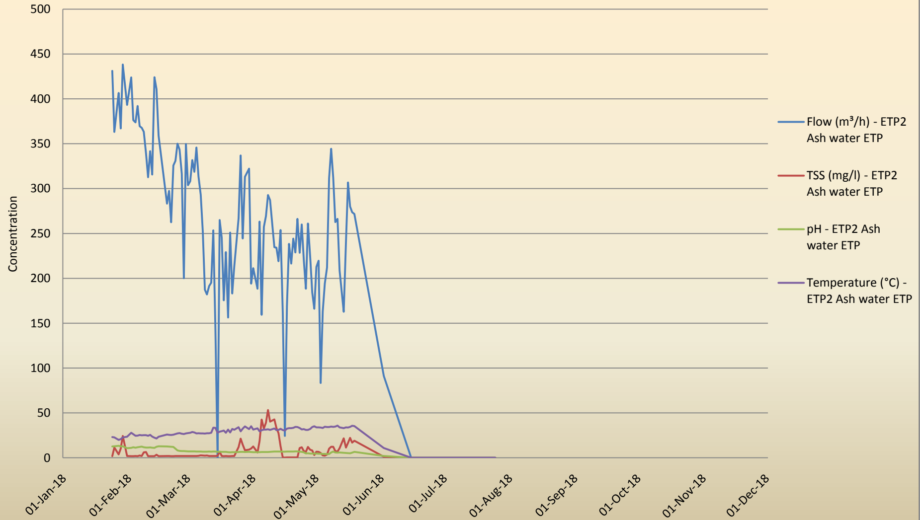
Annual Effluent Trend in M/s. Amarkantak Thermal Power Station, Dist. Anuppur (M.P.)
